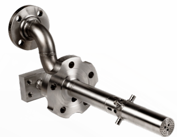
6B SECONDARY FUEL NOZZLE
